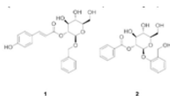
Fig. 1. Structures of compounds 1 and 2.
