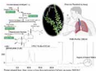
Fig. 1. Steroid-rich fraction isolation scheme, HPLC, and NMR chemical profile
