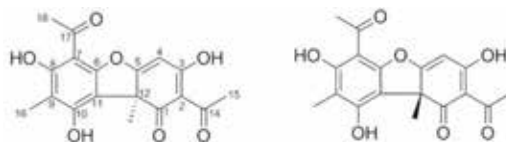
Fig. 1. Structures of usnic acid enantiomers: (-)-usnic acid (left) and (+)-usnic acid (right)
