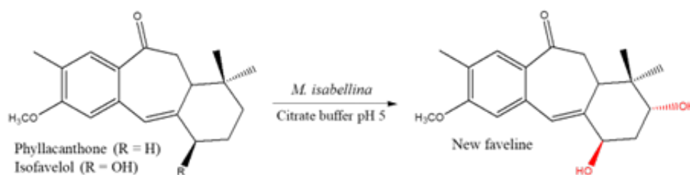
Fig. 1. Biotransformation of phyllacanthone by the fungus M. isabellina NRRL 1757.
