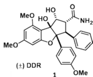
Fig. 1. Structure of (±)-didesmethylocaglamide ( 1 )
