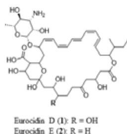
Fig. 1. Structures of eurocidin D (1) and eurocidin E (2)
