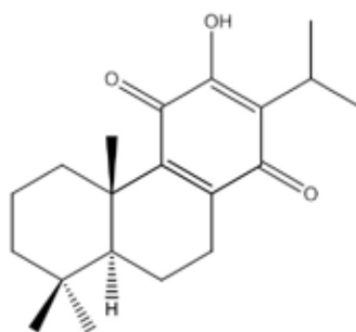
Fig. 1. Royleanone 1 structure
