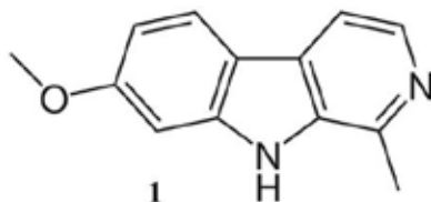
Fig. 1. Structure of harmine (1)
