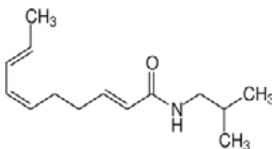
Fig. 1. Structure of spilanthol 1
