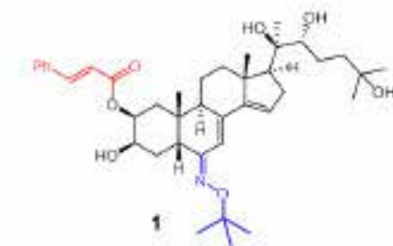
Fig. 1. Structure of the most active ecdysteroid derivative 1
