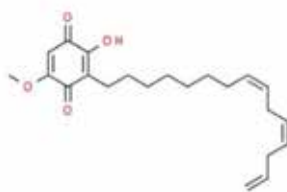
Fig. 1. Structure of sorgoleone 1.
