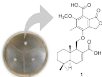
Fig. 1. Structure of new sesquiterpene-phthalide hybrids 1 .
