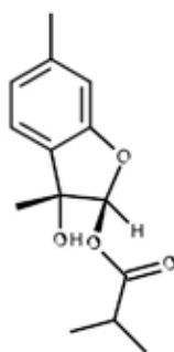
Fig. 1. Structure of a new dihydrobenzofuran derivative 1
