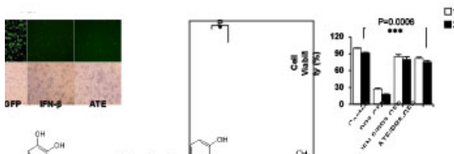
Fig. 1. Antiviral effect of Aster tataricus in RAW264.7 cells and structures of HPLC analysis identified active compounds in the aqueous fraction
