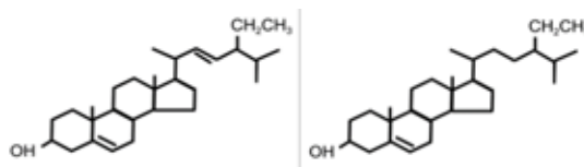
Fig. 1: Structures of stigmasterol and \beta -sitosterol.
