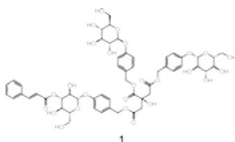
Fig. 1. Structure of sedishin A.
