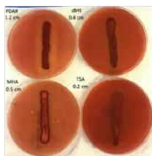
Fig. 1. Modified “agar overlay assay” showing Sa_LaEp14 (seeded in the middle) forming an inhibition halo against Pg.
