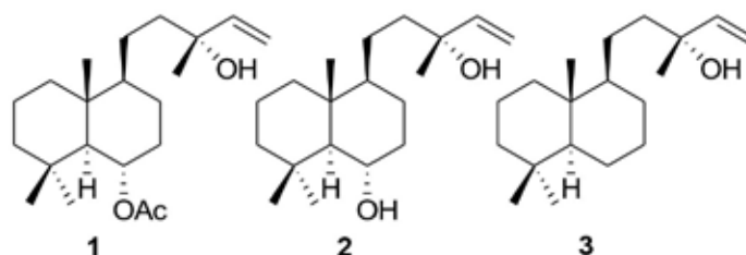
Fig. 1. Structures of larixyl acetate ( 1 ), larixol ( 2 ) and epimanool ( 3 )
