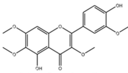
Fig. 1. Structure of the polymethoxyflavone Chrysosplenetin
