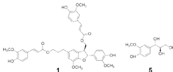
Fig. 1. Two anti- H. pylori compounds isolated from S. williamsii
