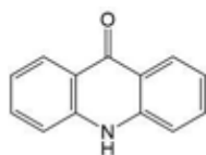
Fig. 1. Structural framework of acridone alkaloid
