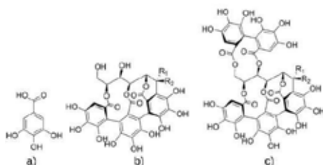
Fig. 1. Structural formula of a) gallic acid, b) vescalal ( R_1=H , R_2=OH ) and castalal ( R_1=OH , R_2=H ) and c) vescalagin ( R_1=H , R_2=OH ) and castalagin ( R_1=OH , R_2=H ).
